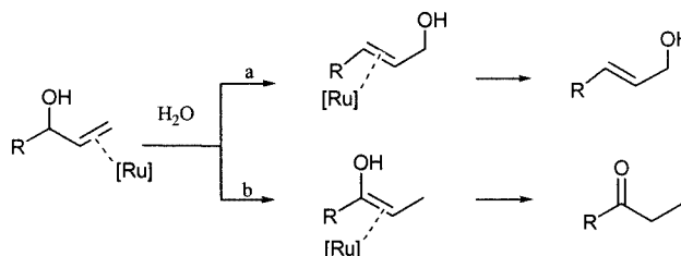
Figure 1. Ruthenium-catalyzed olefin migration in water
