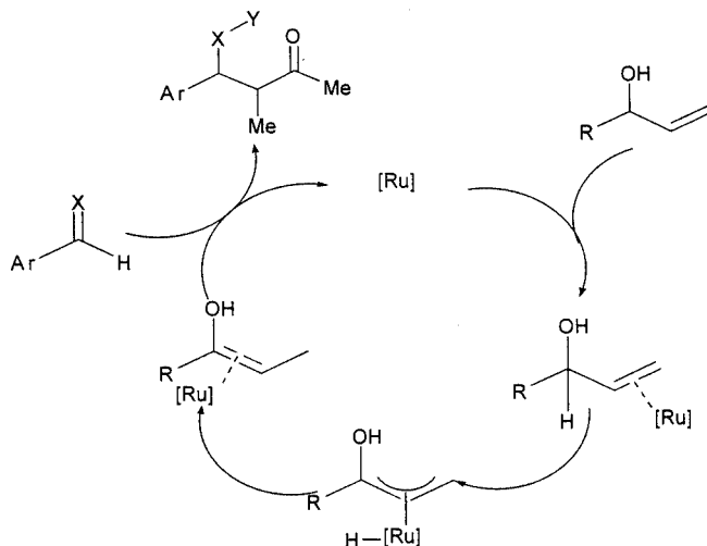
Figure 2. Tentative mechanism for the ruthenium-catalyzed Aldol-type or Mannich-type reactions (R = Me or Ph; X = O or p -MeOC 6 H 4 N; Y = H)
